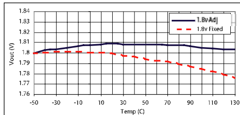
图 8 V IN =3.3V, I OUT =10mA
