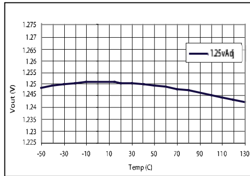
图 6 V out vs 温度, V IN =2.5V, I OUT =10mA
