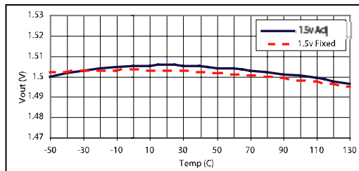
图 7 V IN =3.0V, I OUT =10mA
