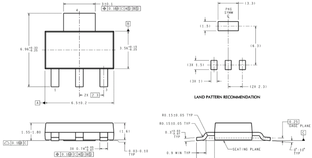
3-Lead SOT-223
