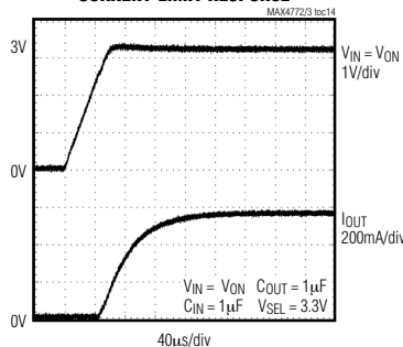
CURRENT-LIMIT RESPONSE
