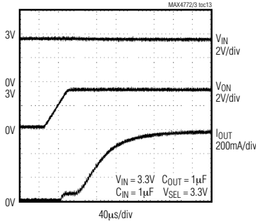
CURRENT-LIMIT RESPONSE
