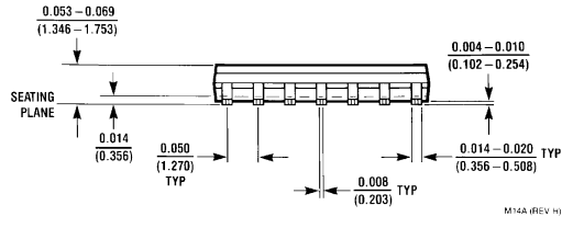
14-Lead Small Outline Molded Package (M) Order Number DM74LS09M NS Package Number M14A
