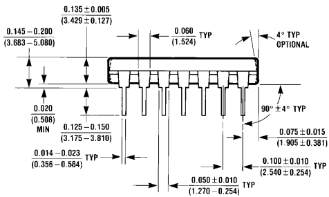
14-Lead Molded Dual-In-Line Package (N) Order Number DM74LS09N NS Package Number N14A
