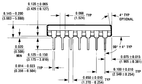
14-Lead Molded Dual-In-Line Package (N) Order Number DM74LS21N NS Package Number N14A
