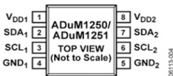
8-LEAD STANDARD SMALL OUTLINE PACKAGE [SOIC_N] NARROW BODY (R-8)
