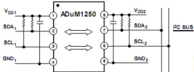
Figure 9. Typical Isolated I 2 C Interface Using ADuM1250
