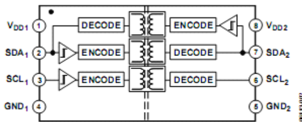
Figure 2. ADuM1251
