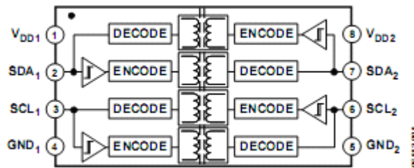
Figure 1. ADuM1250
