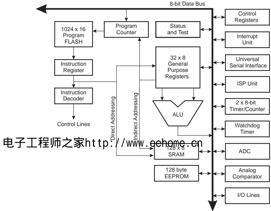
Figure 2. ATtiny26(L) AVR 增强 RISC 结构
