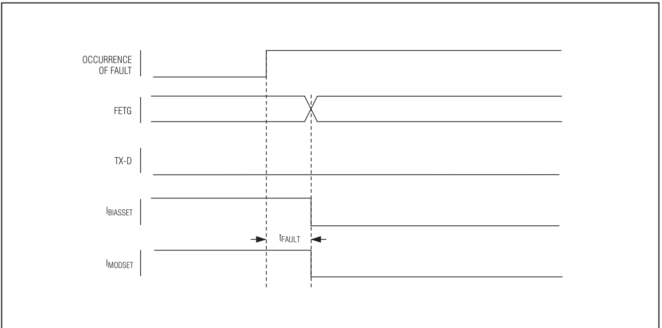
图4. 故障状态检测
