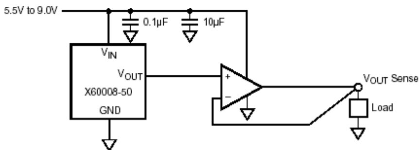
Kelvin Sensed Load
