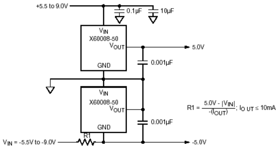
±5.0V Dual Output, High Accuracy Reference
