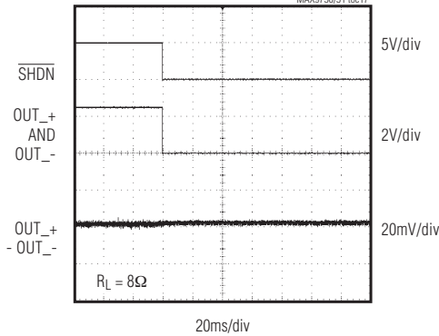
TURN-OFF RESPONSE (SPEAKER MODE)
