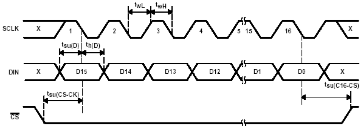
Figure 1. Timing Diagram
