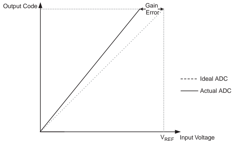
Figure 48. 增益误差
