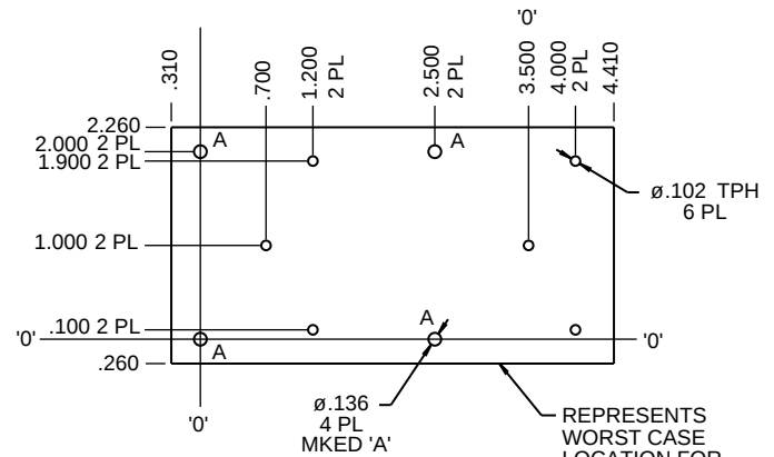
RECOMMENDED CUSTOMER MOUNTING (TOP VIEW)
