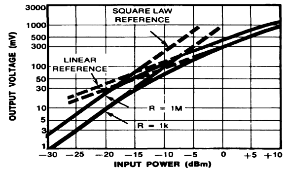
Response Function 2086-6000-00
