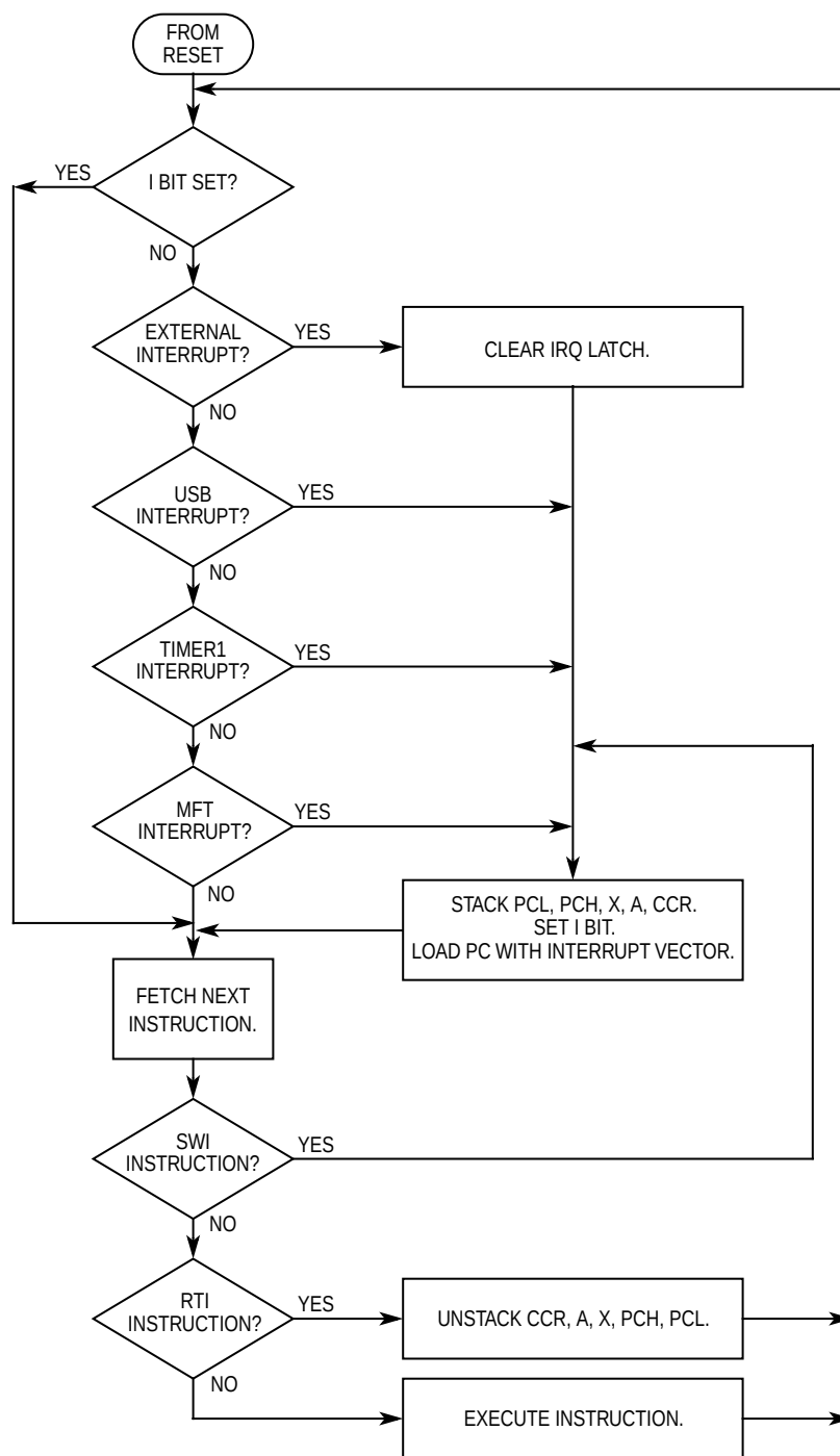
Figure 4-2. Interrupt Flowchart
