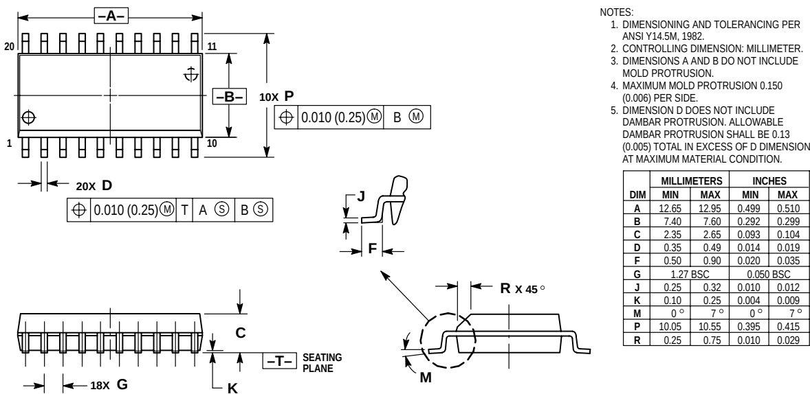
Figure 14-3. 20-Pin SOIC Mechanical Dimensions
