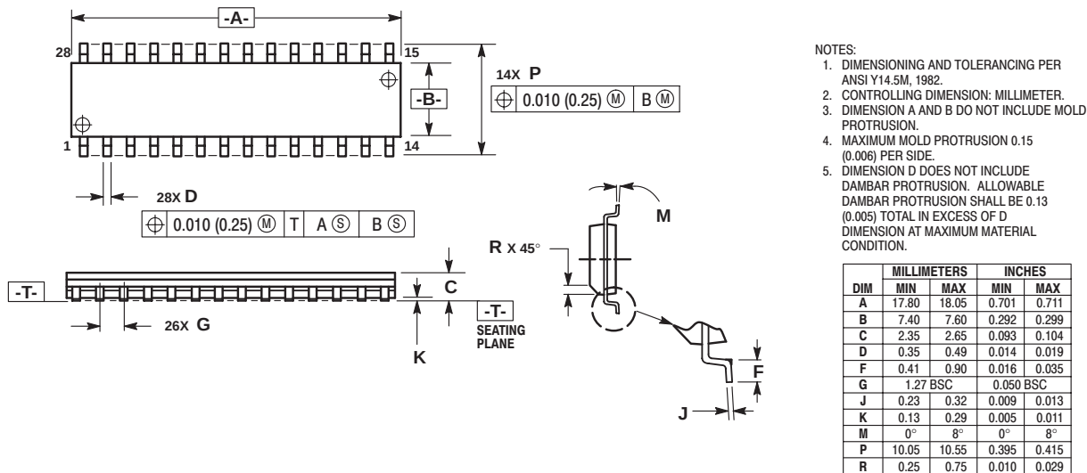
Figure 14-4. 28-Pin SOIC Mechanical Dimensions
