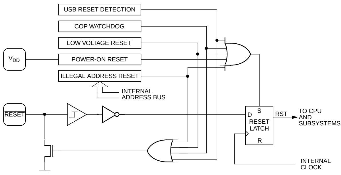
Figure 5-1. Reset Sources
