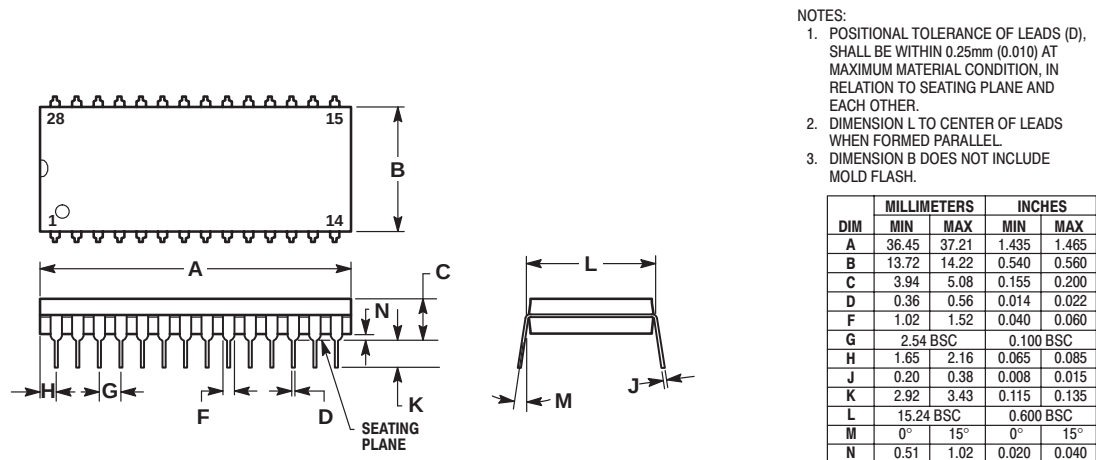
Figure 14-2. 28-Pin PDIP Mechanical Dimensions
