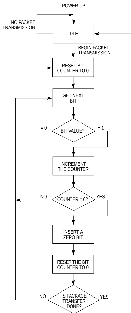
Figure 10-19. Flow Diagram for Bit Stuffing
