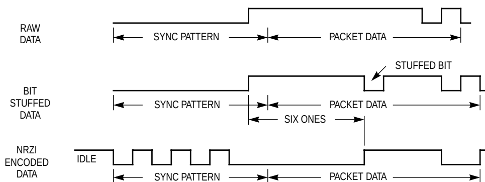
Figure 10-18. Bit Stuffing
