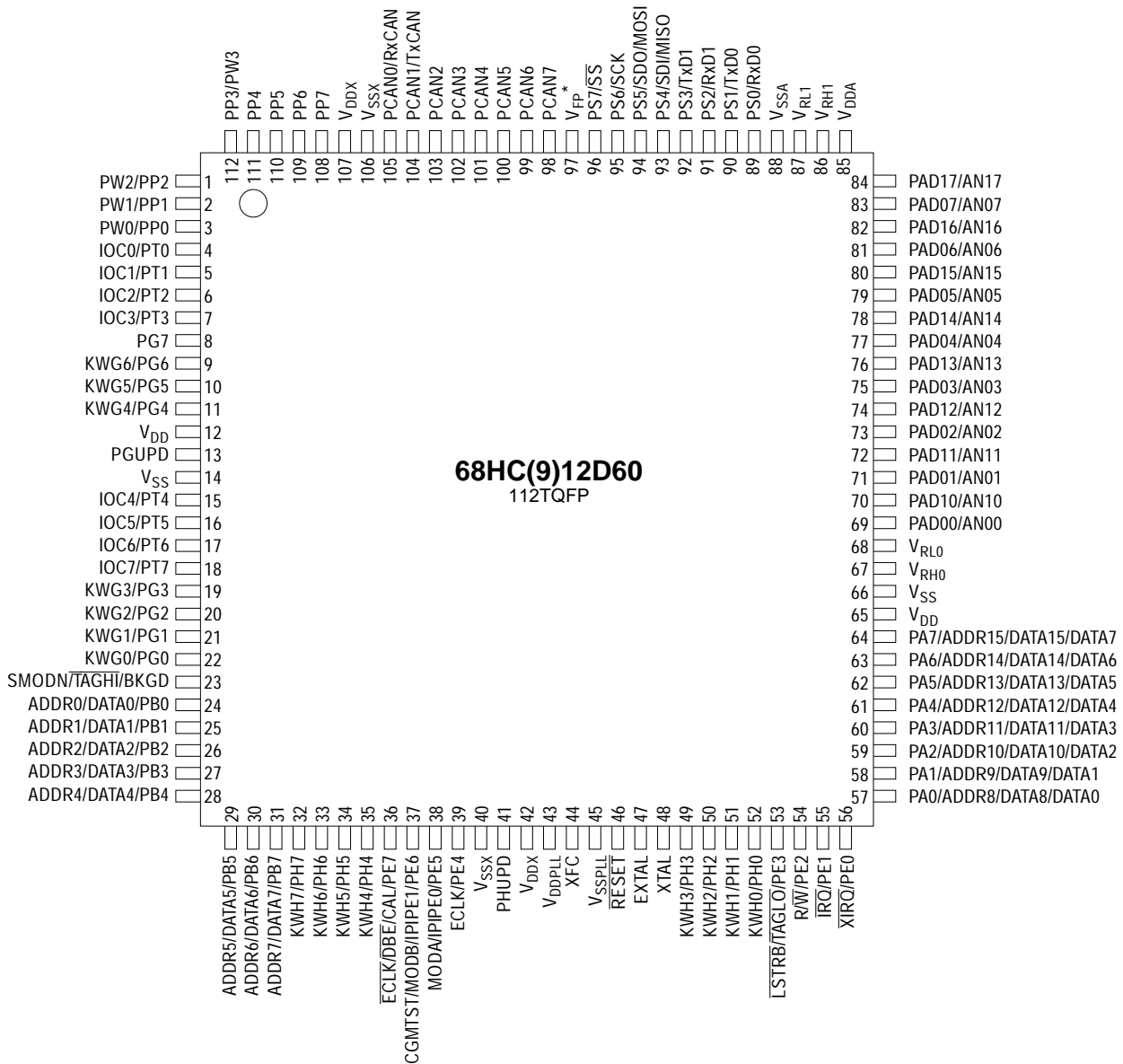
Figure 4 Pin Assignments in 112-pin TQFP for 68HC(9)12D60
