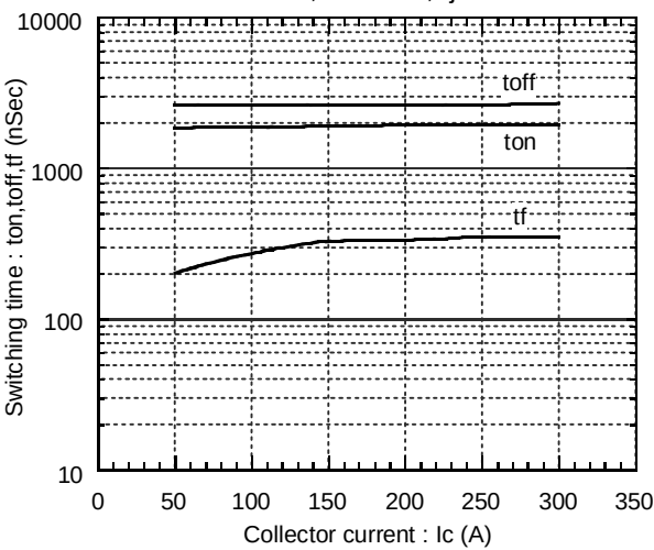
Switching time vs. Collector current E_{dc}=300\text{V}, V_{cc}=15\text{V}, T_j=125^{\circ}\text{C}
