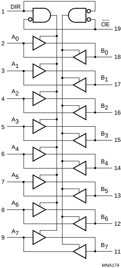
Fig.2 Logic symbol.
