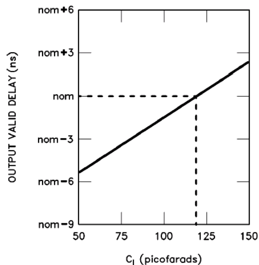
FIGURE 8. TYPICAL OUTPUT VALID DELAY VERSUS LOAD CAPACITANCE AT MAXIMUM OPERATING TEMPERATURE ( C_L = 120 pF)
