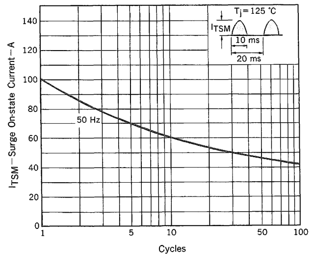
Fig. 2 I_{TSM} RATING
