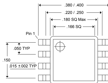
Figure 1. Package Drawings
