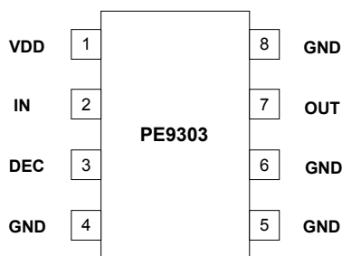
Figure 2. Pin Configuration
