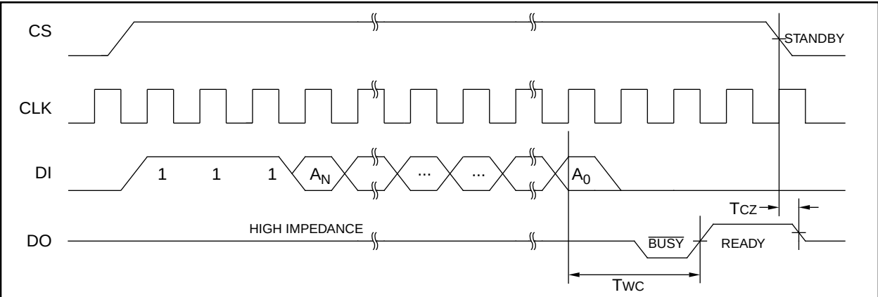
FIGURE 3-7: ERASE
