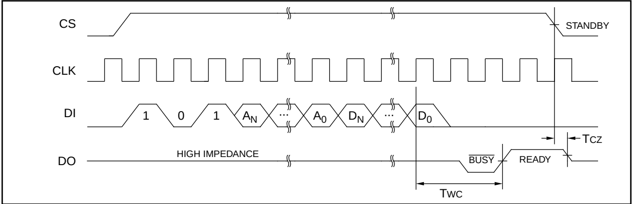
FIGURE 3-6: WRAL
