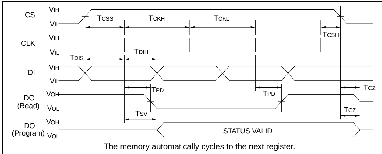
FIGURE 3-2: READ
