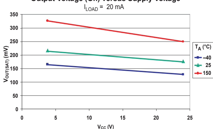
Output Voltage (On) versus Supply Voltage
