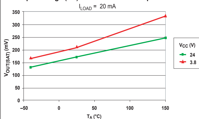
Output Voltage (On) versus Ambient Temperature
