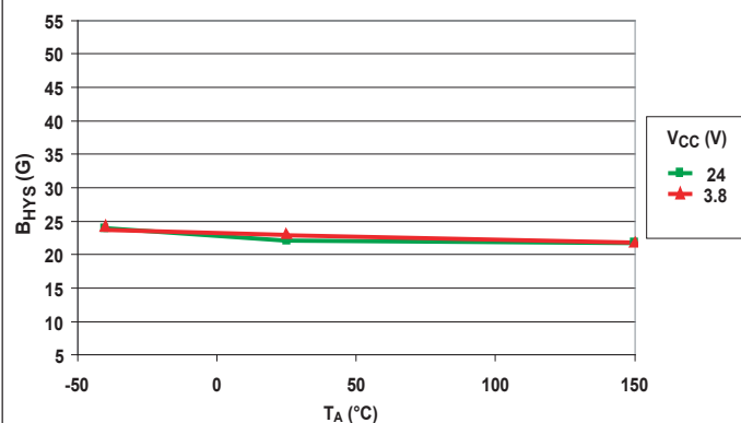
Hysteresis versus Ambient Temperature
