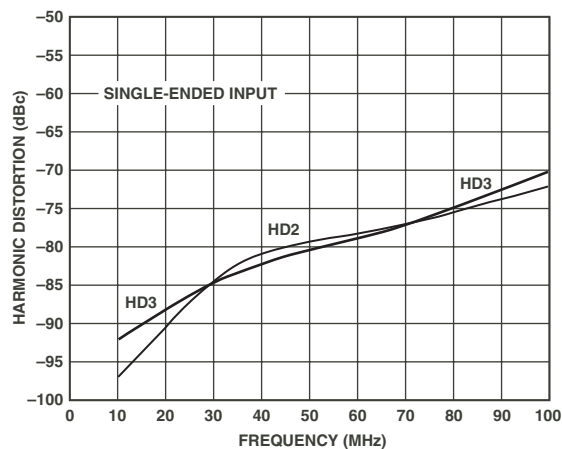
TPC 10. Harmonic Distortion vs. Frequency for 2 V p-p into R_L = 1\text{ k}\Omega Using Single-Ended Input ( A_V = 10\text{ dB} )
