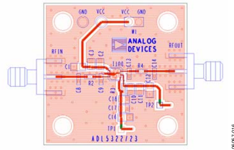
Figure 16. Evaluation Board Component Side View
