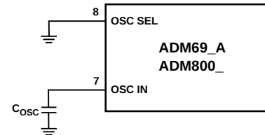
Figure 18c. External Capacitor
