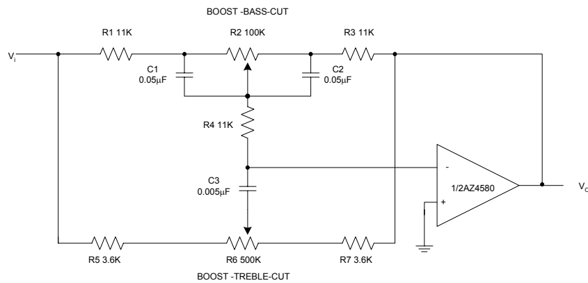
Figure12. Tone Control
