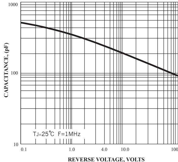
FIG.4-TYPICAL JUNCTION CAPACITANCE
