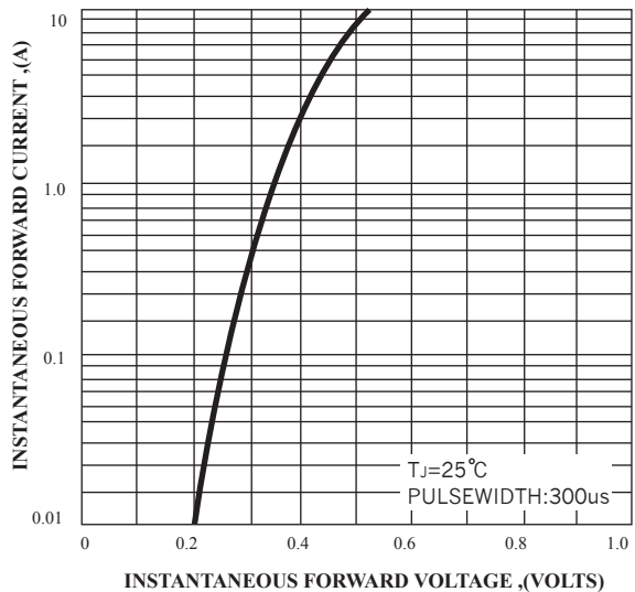
FIG.3-TYPICAL FORWARD CHARACTERISTICS
