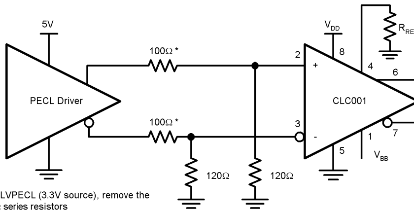
FIGURE 8. PECL, DC-coupled
