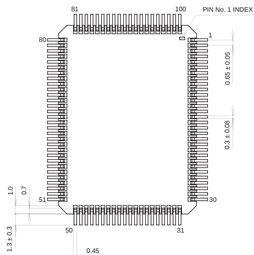
PACKAGE STRUCTURE
