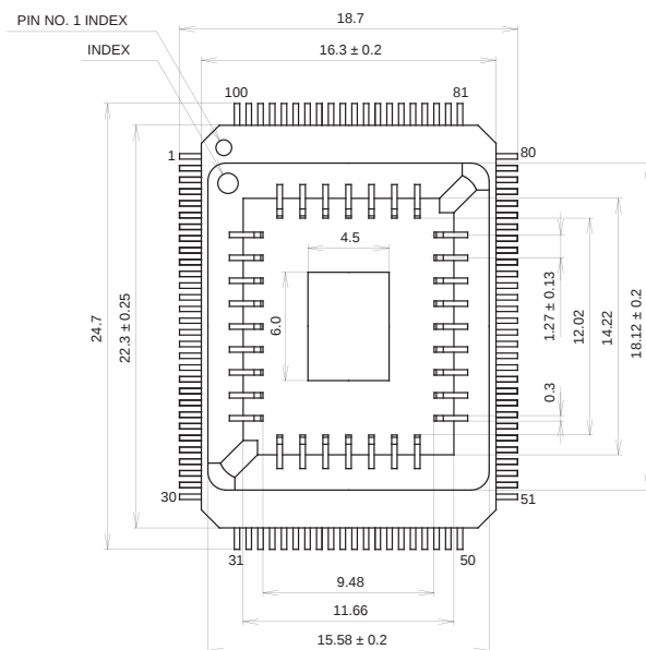
100PIN PQFP (CERAMIC)
