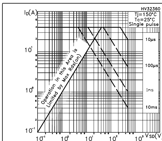
Figure 5. Safe operating area for DPAK / IPAK
