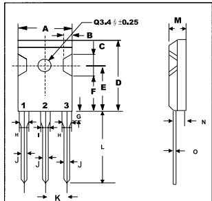
TO-247 (3P)
