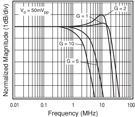
Non-Inverting Freq. Response, V_S = 1.2\text{V}
