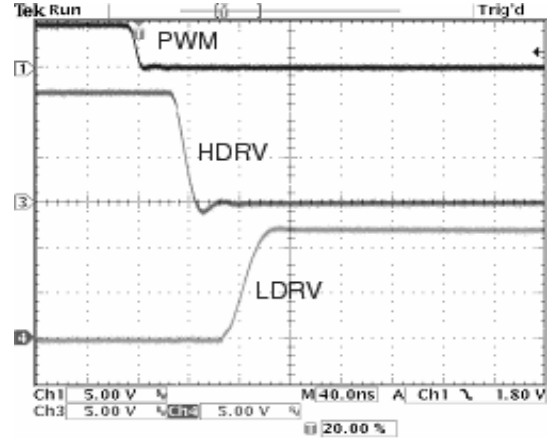
Gate Drive Rise and Fall Times (2)
