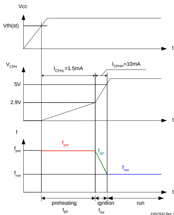
Figure 17. Operating Modes
