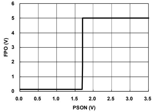
Figure 1. \overline{\text{PSON}} Threshold Voltage
