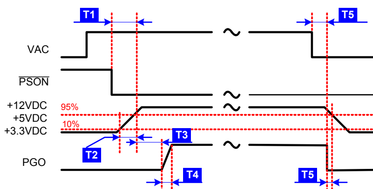
Figure 1. Timing Diagram
