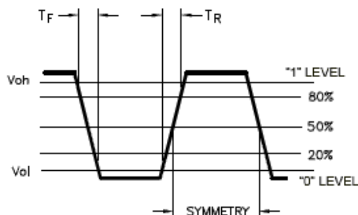
OUTPUT WAVEFORM
