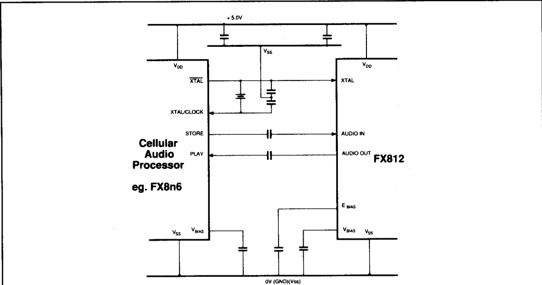
Fig.3 Interfacing to an Audio Processor
