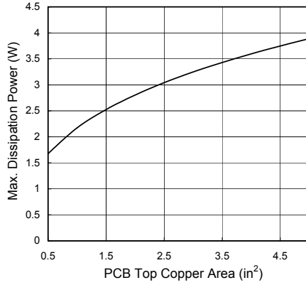
G1084T53(TO-263) Max. Power Dissipation vs. PCB Top Copper Area Area T_{AMB} = 25^{\circ}\text{C} ; Still Air
