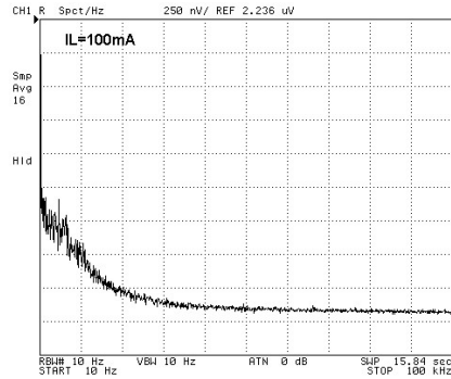
Output Noise
