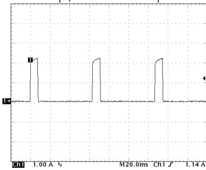
Short Circuit-Current
