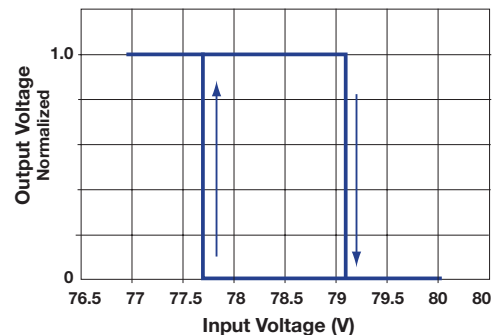
Overvoltage Hysteresis
