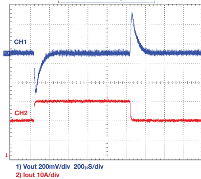
Transient Response
