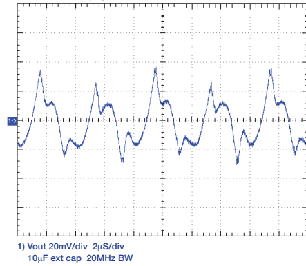
Voltage Ripple
