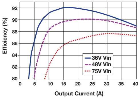
Efficiency
