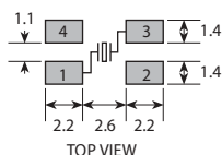
SOLDER PAD LAYOUTS
