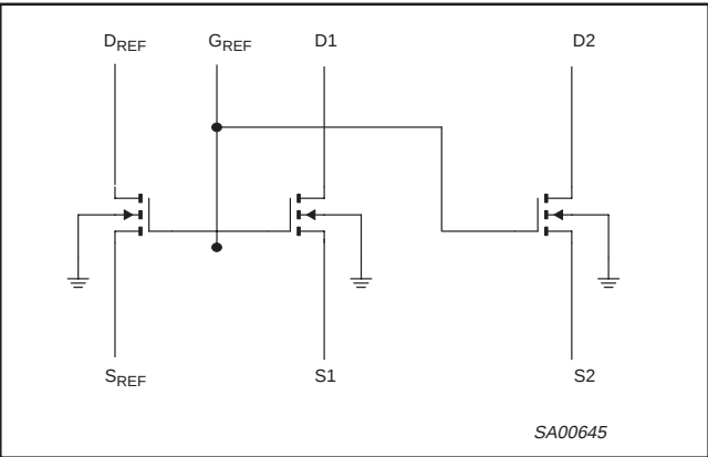
Figure 3. Clamp schematic
