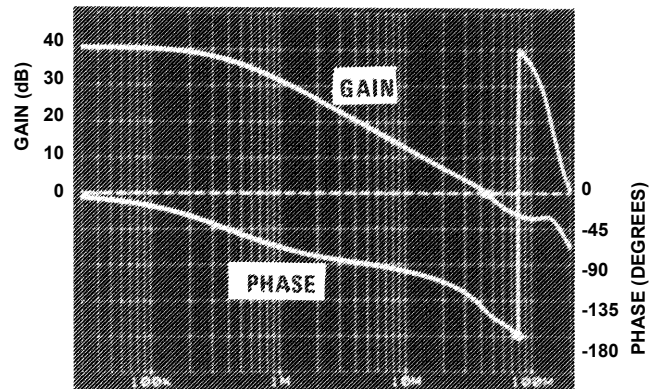
FREQUENCY RESPONSE
