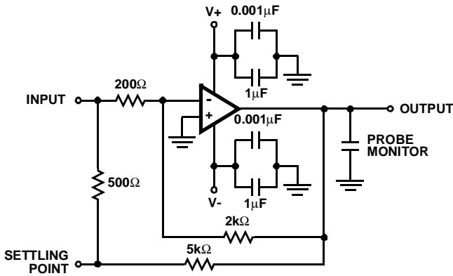
SETTLING TIME TEST CIRCUIT
