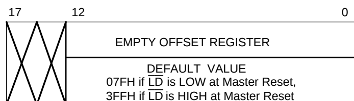
72264 with MAC = GND (8,192 x 18-BIT)
