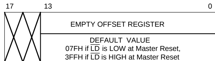
72274 with MAC = GND (16,384 x 18-BIT)
