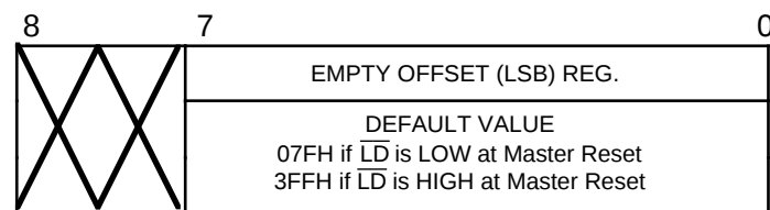
72264 with MAC = Vcc (16,384 x 9-BIT)
