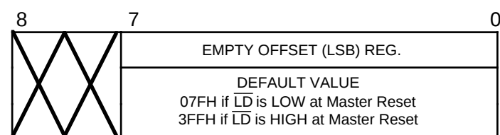
72274 with MAC = Vcc (32,768 x 9-BIT)
