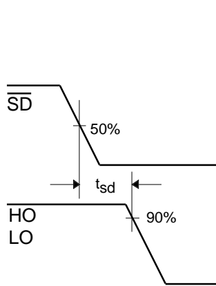
Figure 3. Shutdown Waveform Definitions
