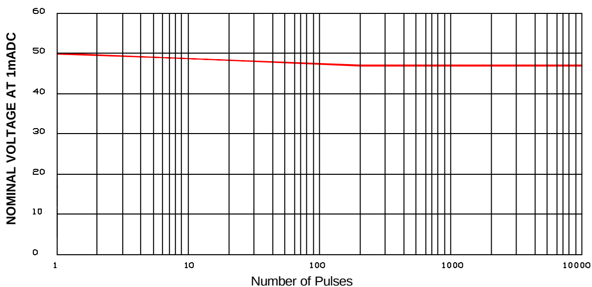
NOMINAL VOLTAGE STABILITY TO MULTIPLE ESD IMPULSES (8KV CONTACT DISCHARGES PER IEC 61000-4-2)
