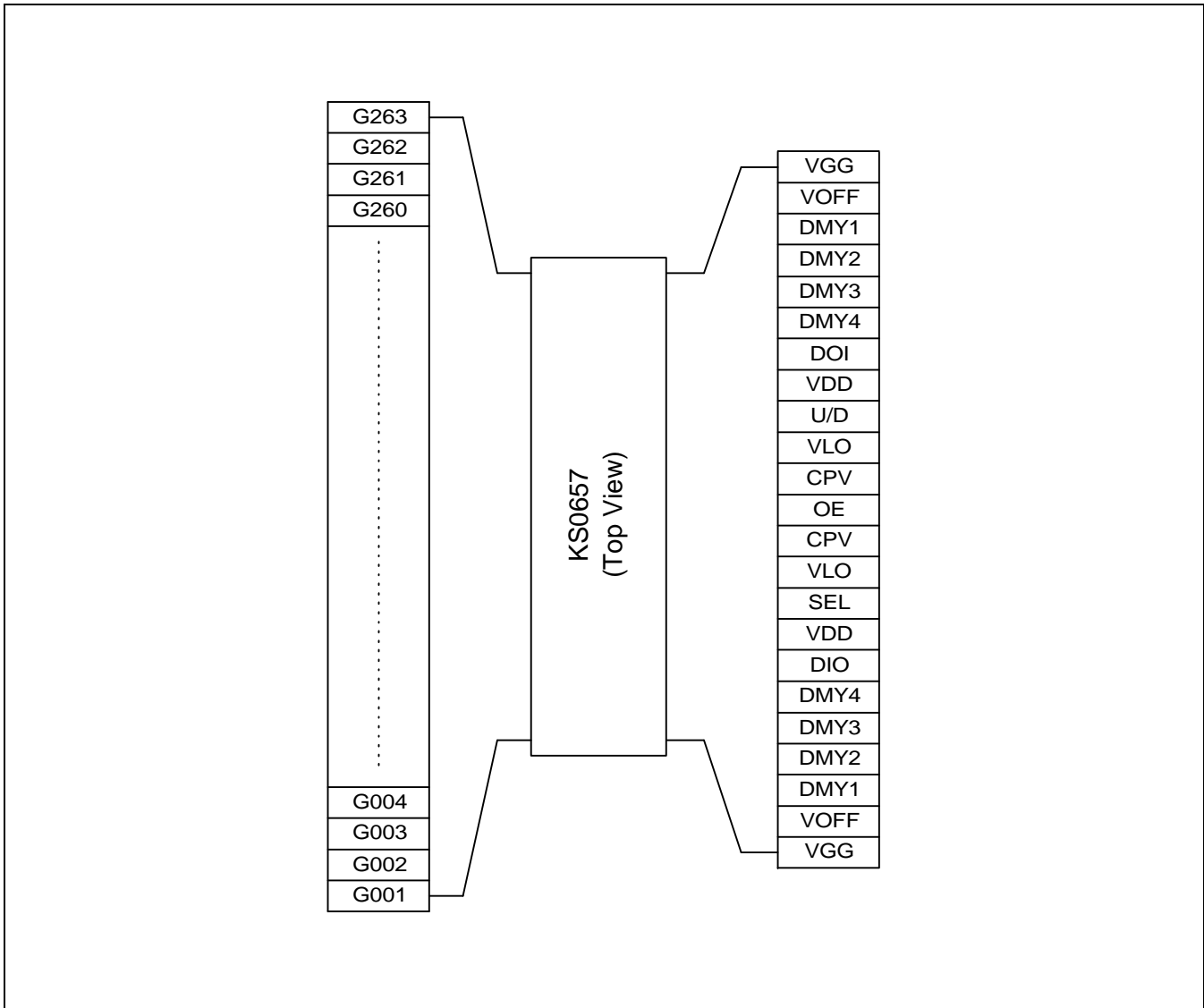
Figure 2. Pin Assignments
