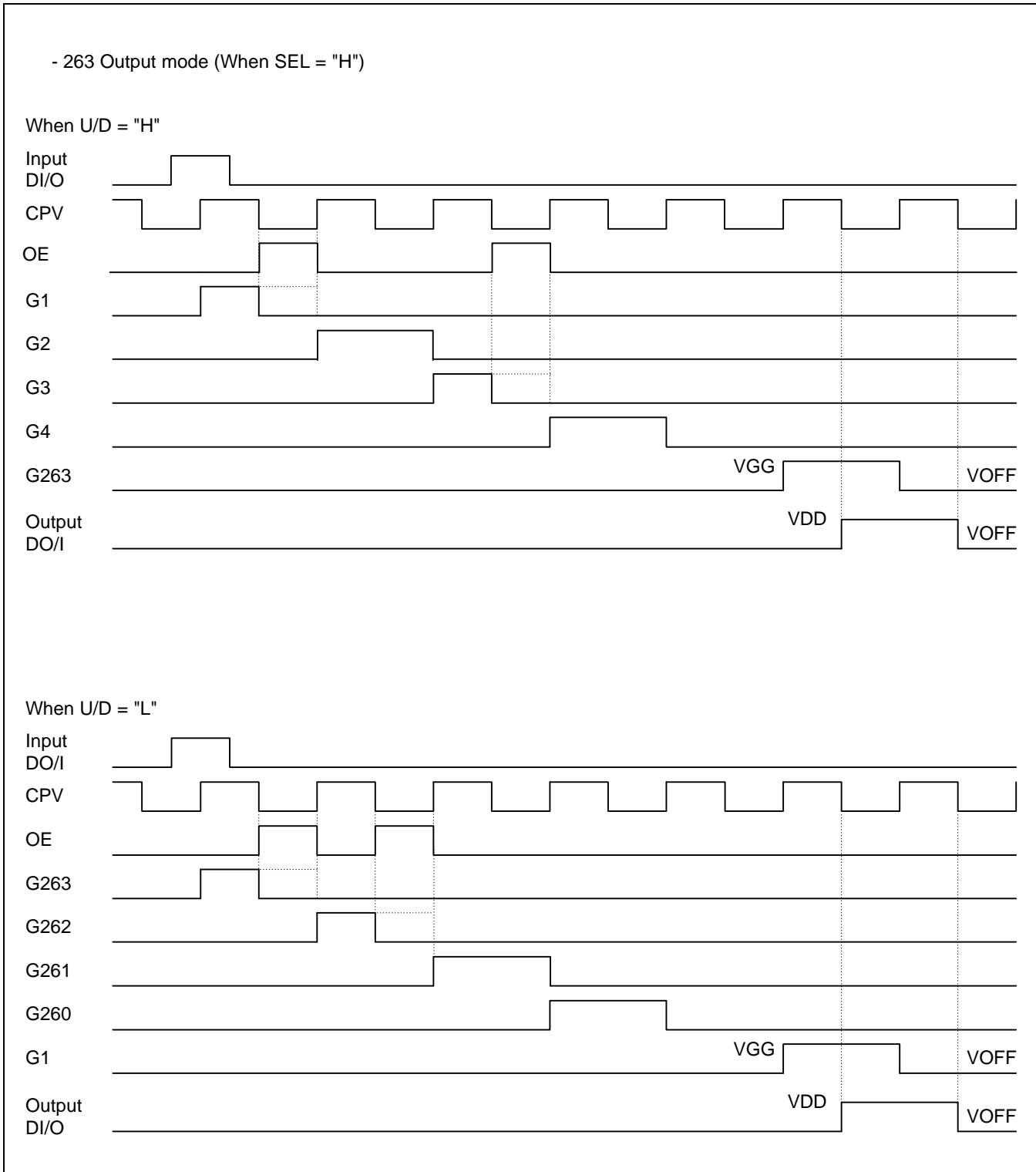
Figure 5. Recommended Timing
