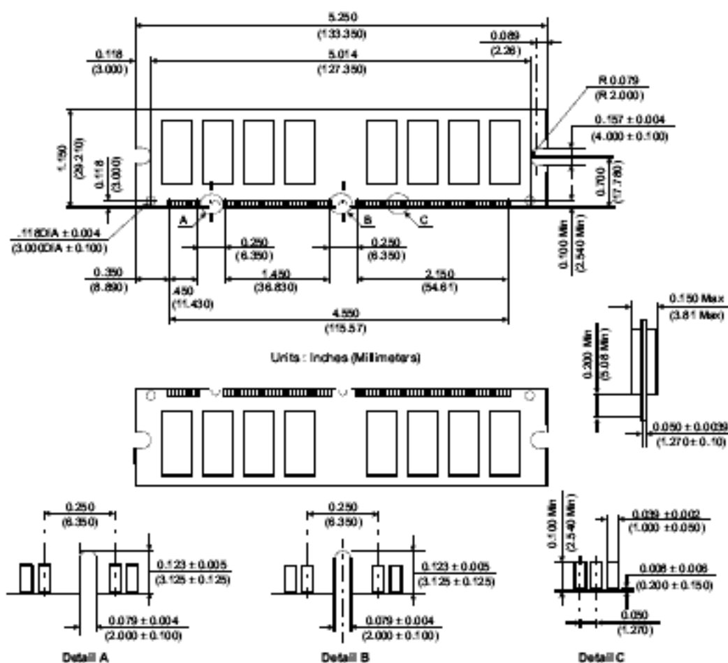
Figure 1: KVR133X64C3/1G 168-Pin SDRAM Module
