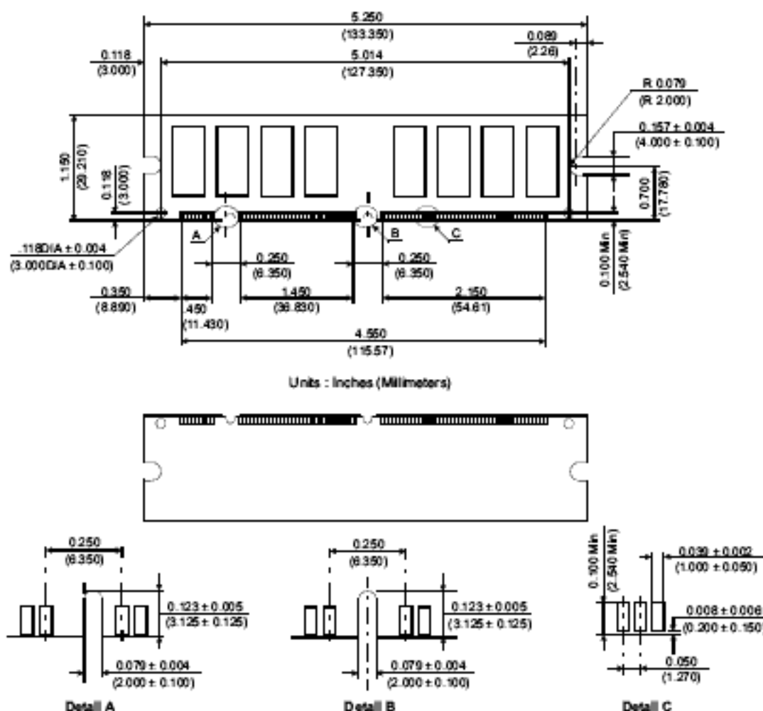
Figure 1: KVR133X64C3L/256 168-Pin SDRAM Module
