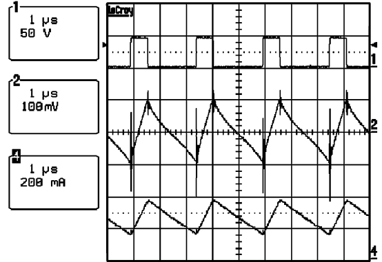
Operational Waveforms
